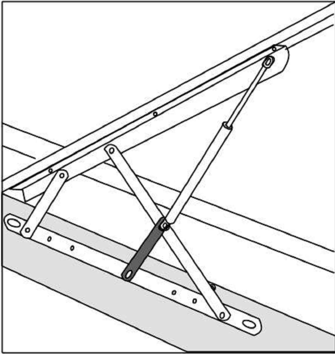
LOCK POSITION
